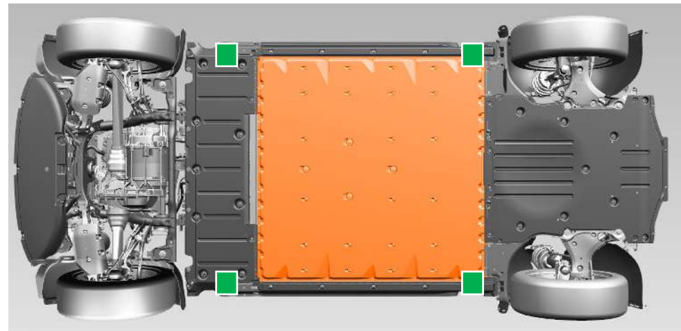
Suitable lifting points on vehicles with a high-voltage drive, e.g. ID.4
