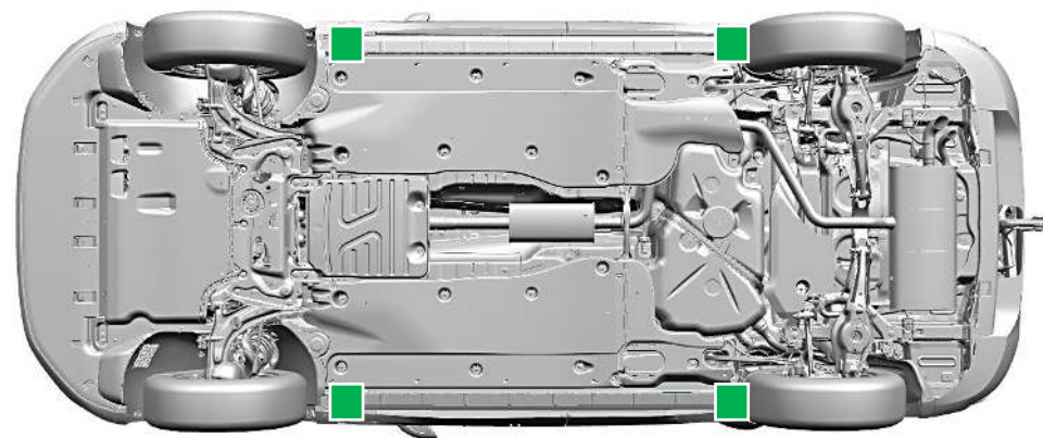
Suitable lifting points on vehicles with a combustion engine drive, e.g. Tiguan
